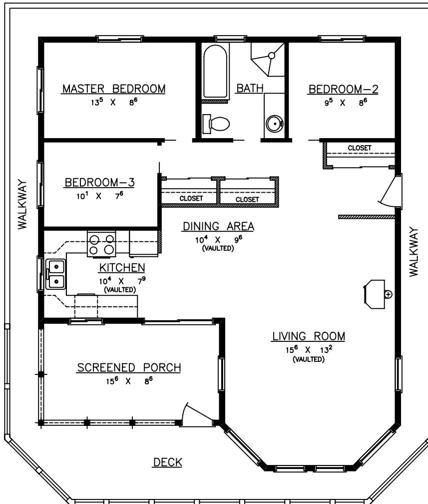
FLOOR PLAN
